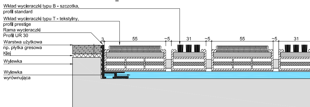
UNIMAT V 22 TB_P + UR 30
