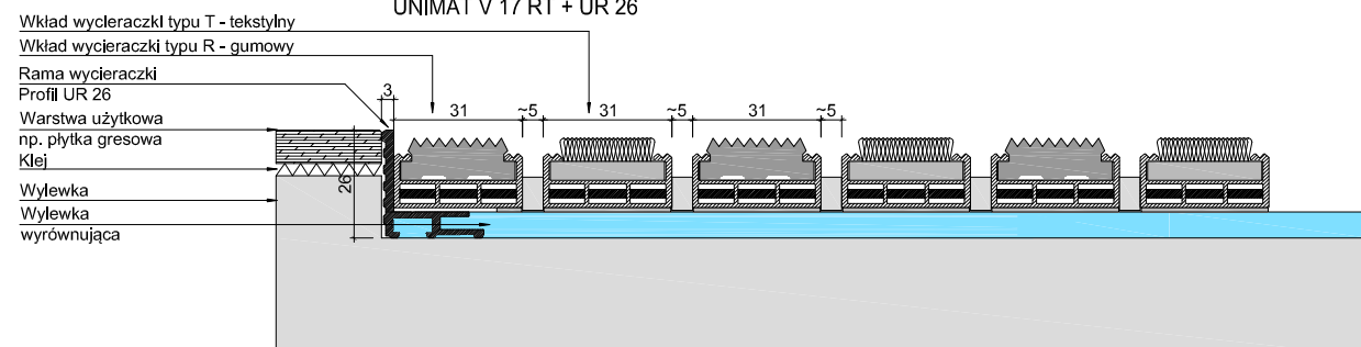
UNIMAT V 17 RT + UR 26
