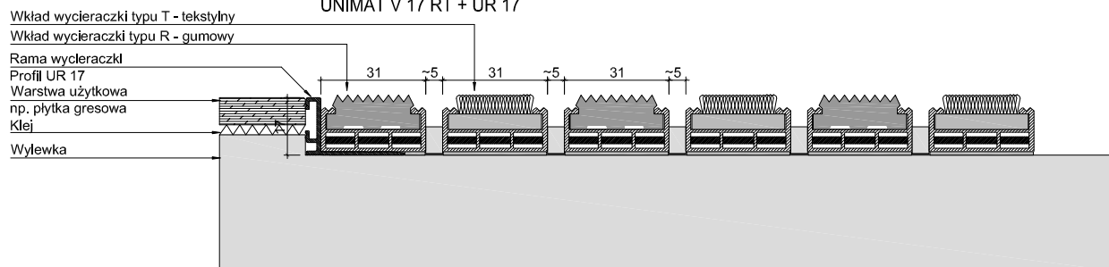
UNIMAT V 17 RT + UR 20
