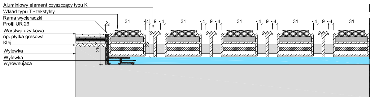
UNIMAT V 22 KT + UR 26
